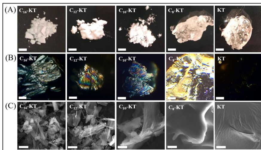
Fig. 4. Images of KT and its conjugates under (A) Visual examination (scale bar = 3 mm), (B) Polarized microscope (scale bar = 50 \mu m), and (C) Scanning electron microscope (SEM) (scale bar = 5 \mu m).
