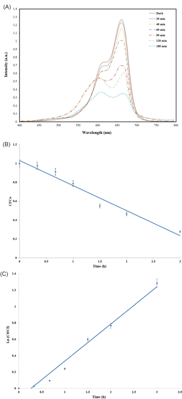
Fig. 6. (A) UV absorption spectra of the MB in the presence of PLGA/10 wt.%TiO 2 nanocomposite, (B) photodegradation of the MB dye, and (C) kinetic curves for photocatalytic degradation of MB under UV irradiation.
