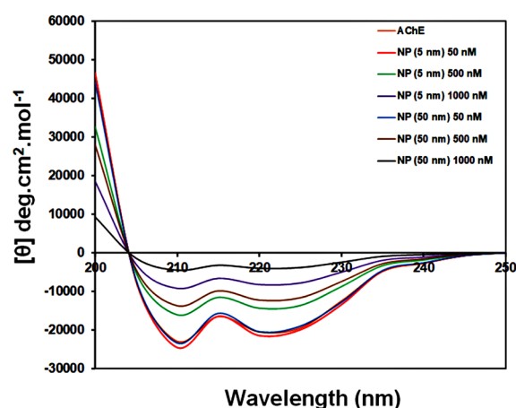
Fig. 5. CD spectra of AChE in the absence and presence of additional concentrations (50, 500, and 1000 nM) of Fe 2 O 3 NPs.
