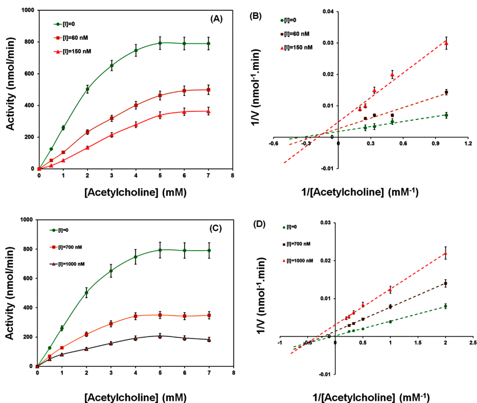
Fig. 3. Michaelis-Menten and Lineweaver-Burk plots of AChE with and without various concentrations of Fe 2 O 3 NPs with 5 nm (A and B) and 50 nm (C and D) in size.
